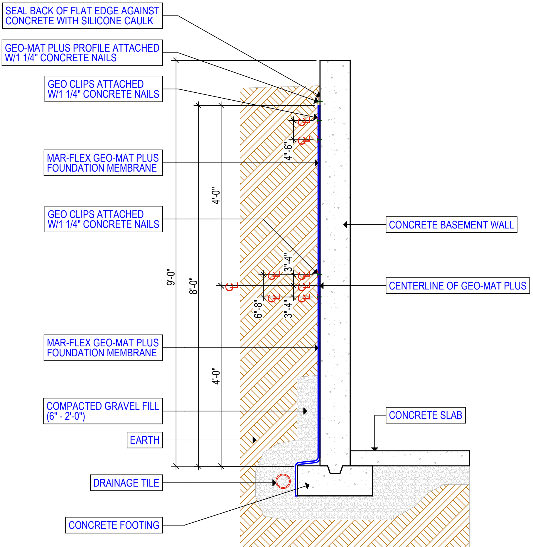
9'-0" WALL DETAIL (8'-0" HIGH GEO-MAT PLUS) GEO-MAT PLUS FOUNDATION WALL SECTION SCALE : 1/2" = 1'-0"
