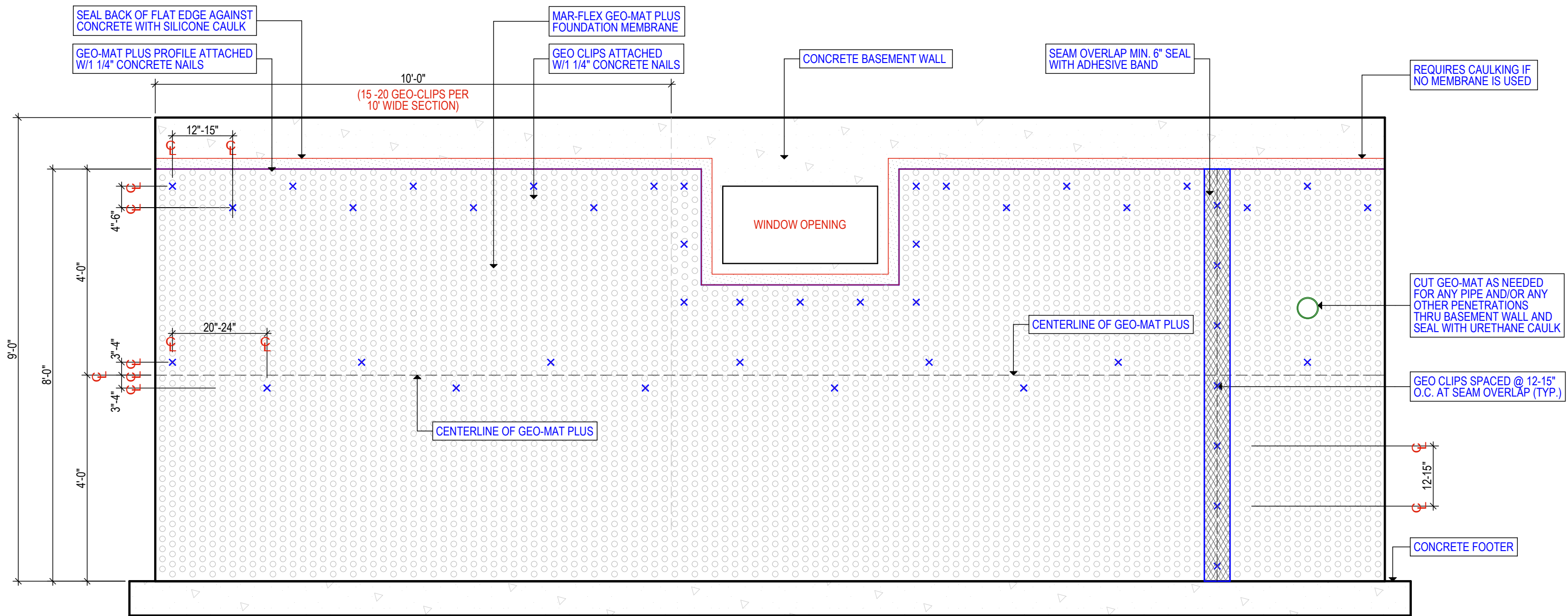
9'-0" WALL DETAIL (8'-0" HIGH GEO-MAT PLUS) GEO-MAT FOUNDATION WALL SECTION SCALE : 1/2" = 1'-0"
