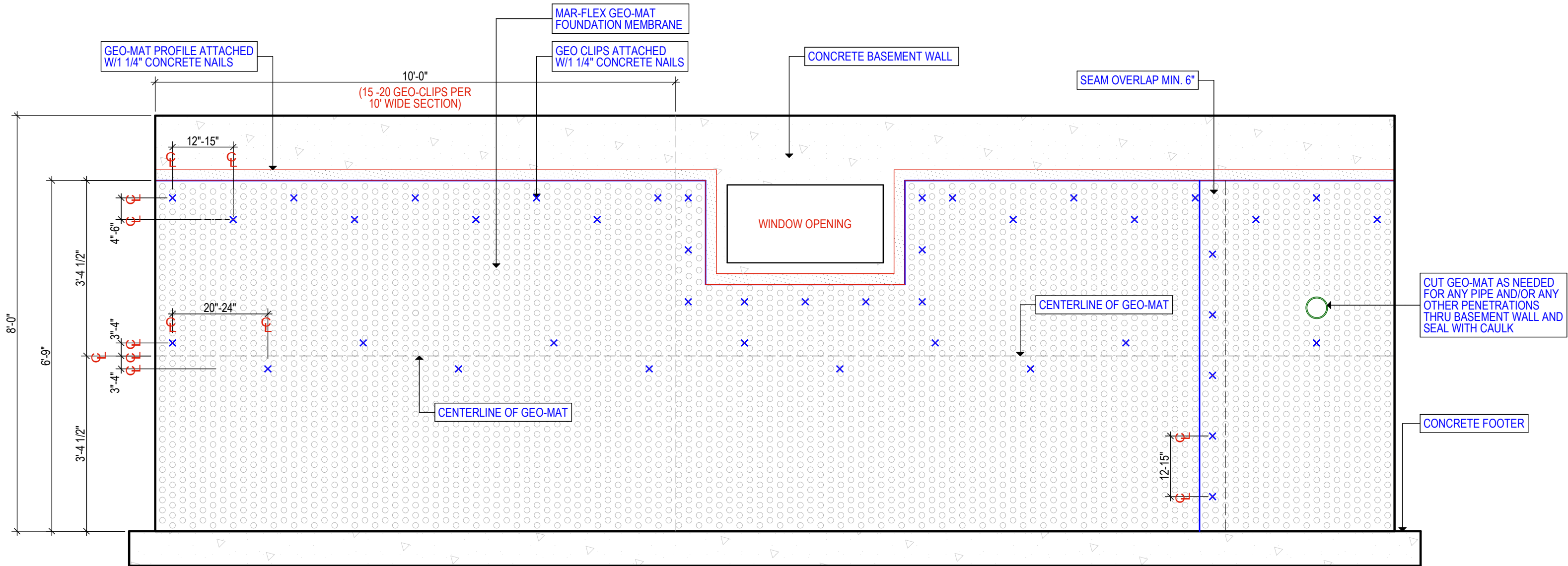
8'-0" WALL DETAIL (6'-9" HIGH GEO-MAT) GEO-MAT FOUNDATION WALL SECTION SCALE : 1/2" = 1'-0"
